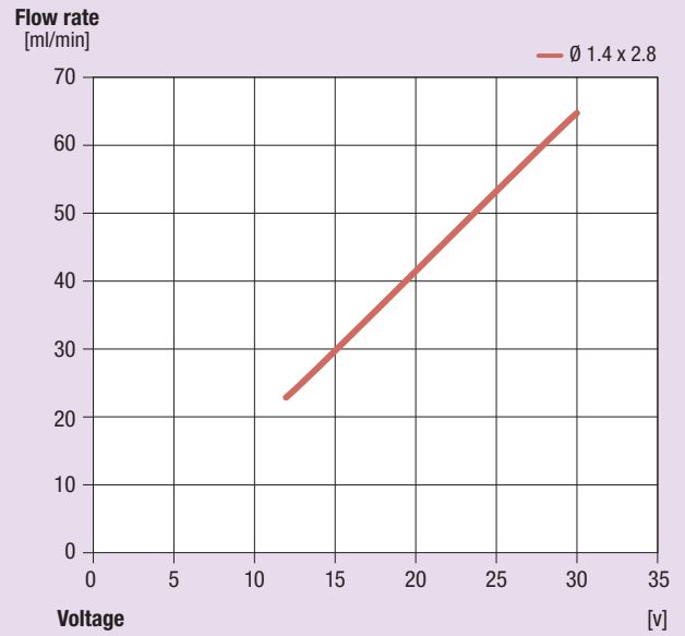
TP16 @ 0 bar
