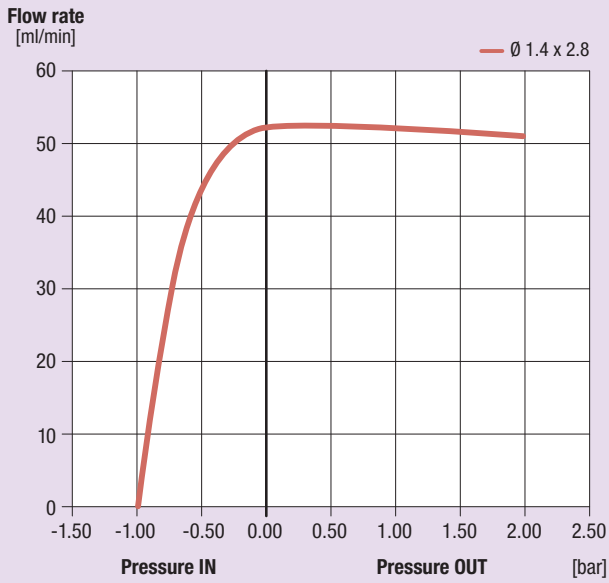
TP16 @ 24 V
